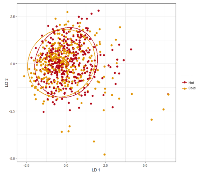
Fig. 4: Linear discriminant analysis of season's effect.
