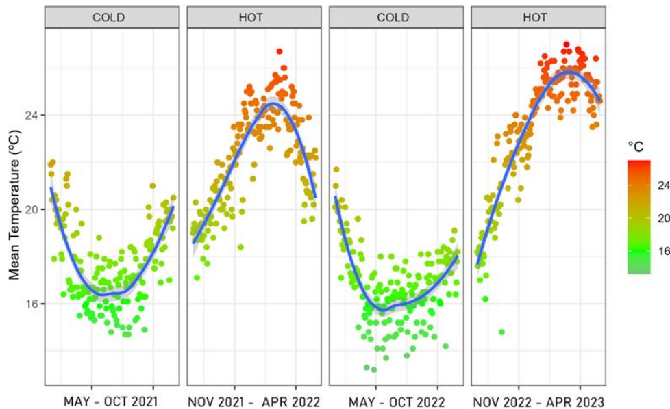
Fig. 1: Mean temperature from May 2021 to April 2023, data were separated into hot and cold seasons.
